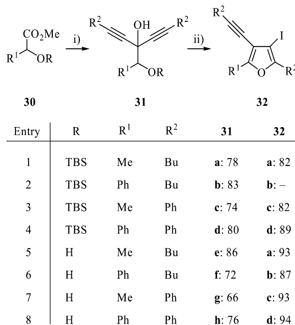
Scheme 10. i) 2 (R = TBS) or 3 (R = H) equiv. R 2 CCLi, THF, -78^{\circ}\text{C} , 1 h; ii) 3 I 2 , 3 NaHCO 3 , MeCN, 20^{\circ}\text{C} , 1 h.
