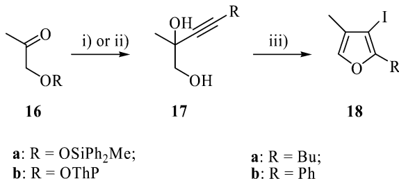
Scheme 6. i) [ 17a ] RCCLi , THF, 0 °C, 2 h then TBAF, THF [89%]; ii) [ 17b ] as i) then p TSA, MeOH, 20 °C, 2 h [71%]; iii) as Scheme 5 [ 18a : 82%; 18b : 61%].
