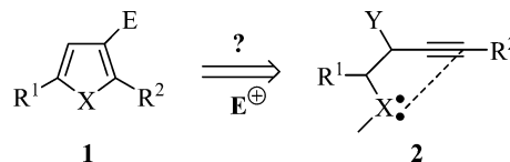
Figure 1. Electrophile-driven 5- endo-dig cyclisation.
