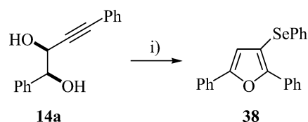
Scheme 12. i) PhSeCl, K 2 CO 3 , THF, –78 °C, 5 h [29%].
