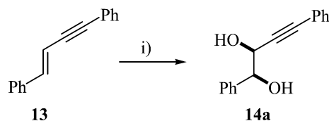
Scheme 4. i) \text{K}_2\text{OsO}_4 \cdot 2\text{H}_2\text{O} (cat.), \text{K}_3\text{Fe}(\text{CN})_6 (xs), \text{K}_2\text{CO}_3 (xs), \text{MeSO}_2\text{NH}_2 , quinuclidine (cat.), t\text{BuOH}/\text{H}_2\text{O} (1:1), 20^\circ\text{C} , 96 h (78%).
