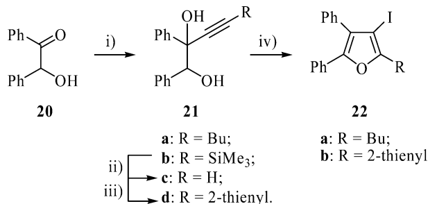
Scheme 7. i) [ 21a , 21b ] 2.1 equiv. RCCLi , THF, -78 °C to 0 °C [68%; 77%]; ii) [ 21c ] TBAF, THF, 0 °C, 20 min. [80%]; iii) 2-iodothiophene, Pd(PPh_3)_4 , Et_2NH , 20 °C, 16 h [81%]; iv) as Scheme 5 [ 22a : 93%; 22b : 71%].
