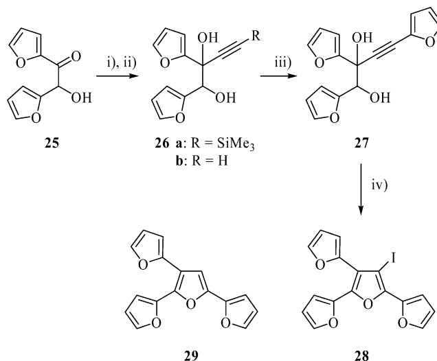
Scheme 9. i) TMSCLi, THF, -78^{\circ}\text{C} to 0^{\circ}\text{C} [78%]; ii) TBAF, THF, 20 min. [68%]; iii) 2-iodofuran, CuI (cat.), Pd(PPh 3 ) 4 (cat.), Et 2 NH, 20^{\circ}\text{C} , 16 h [74%]; iv) 3I 2 , 3NaHCO 3 , dry EtOAc, 20^{\circ}\text{C} , 1 h [25%].
